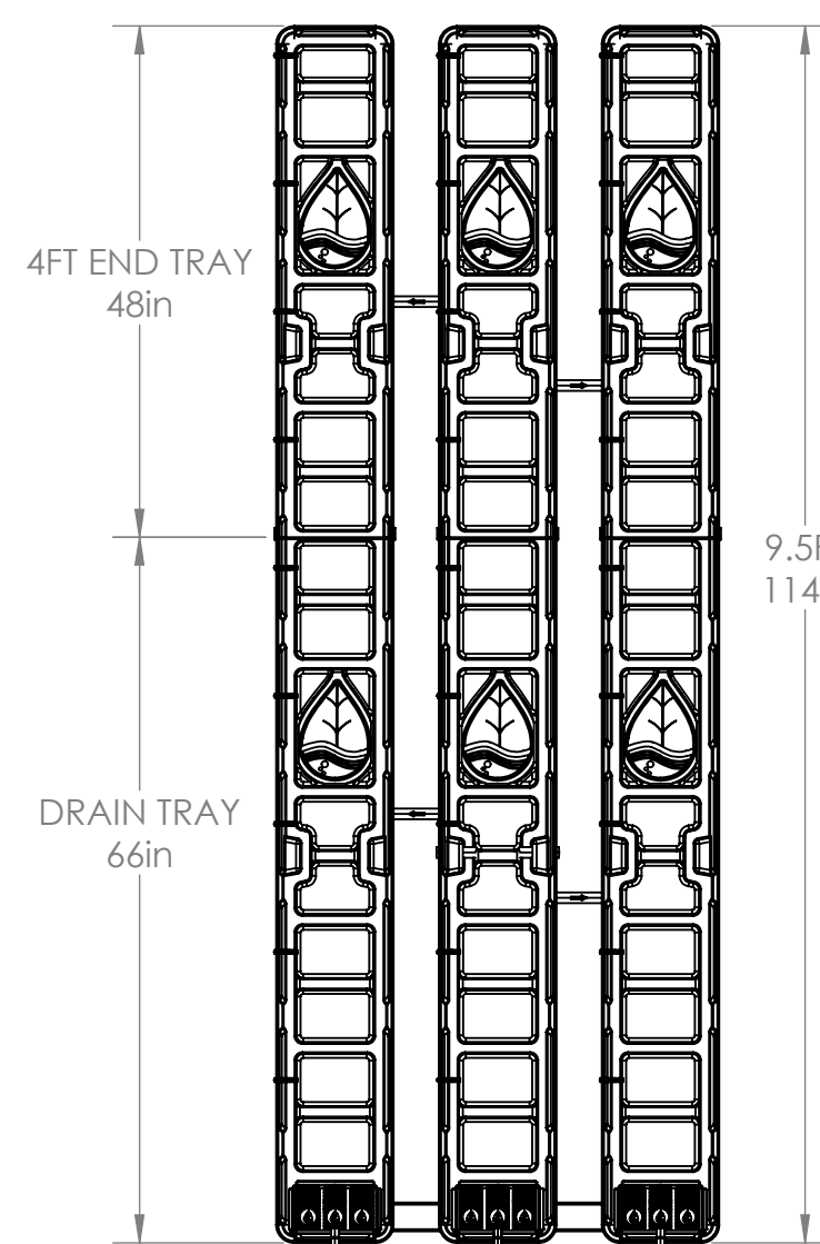
3 TRAYS WIDE (FOR 4FT WIDE BOTANICARE BENCH)
