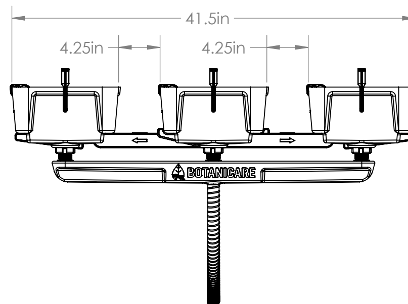
3 TRAYS WIDE (FOR 4FT WIDE BOTANICARE BENCH)
