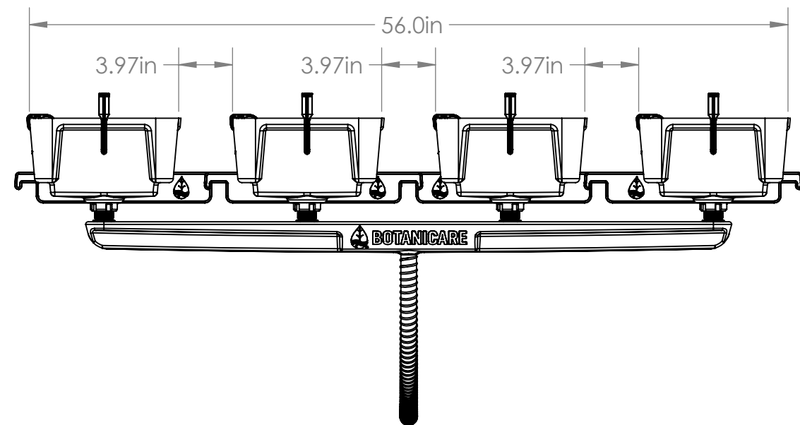
4 TRAYS WIDE (FOR 5FT WIDE BOTANICARE BENCH)
